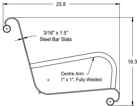
Seat Section Profile Detail
